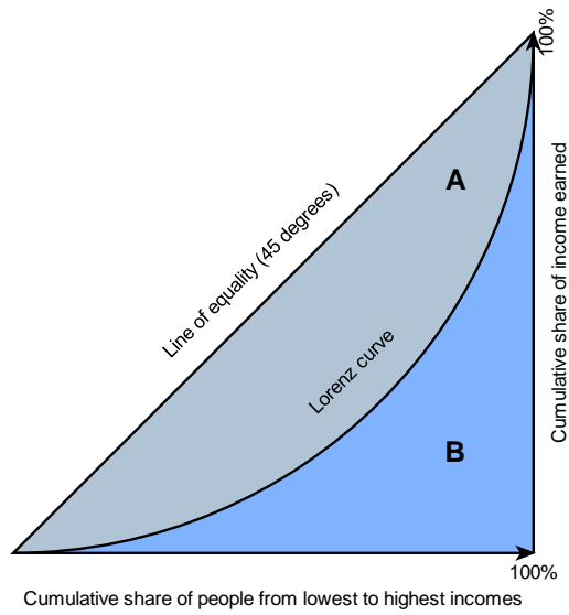
Figure 7: Lorenz Curve 4
